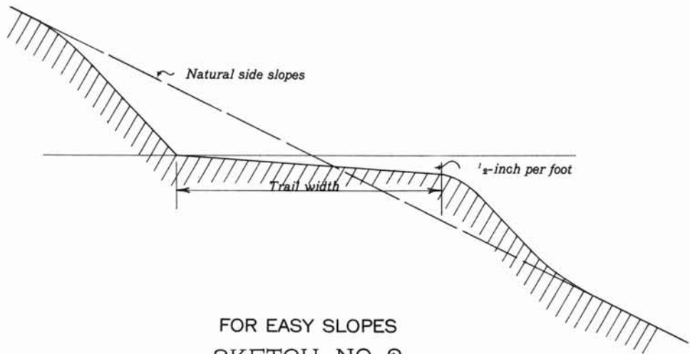
A GOOD CROSS SECTION IN HEAVY CUT SKETCH NO. 1
