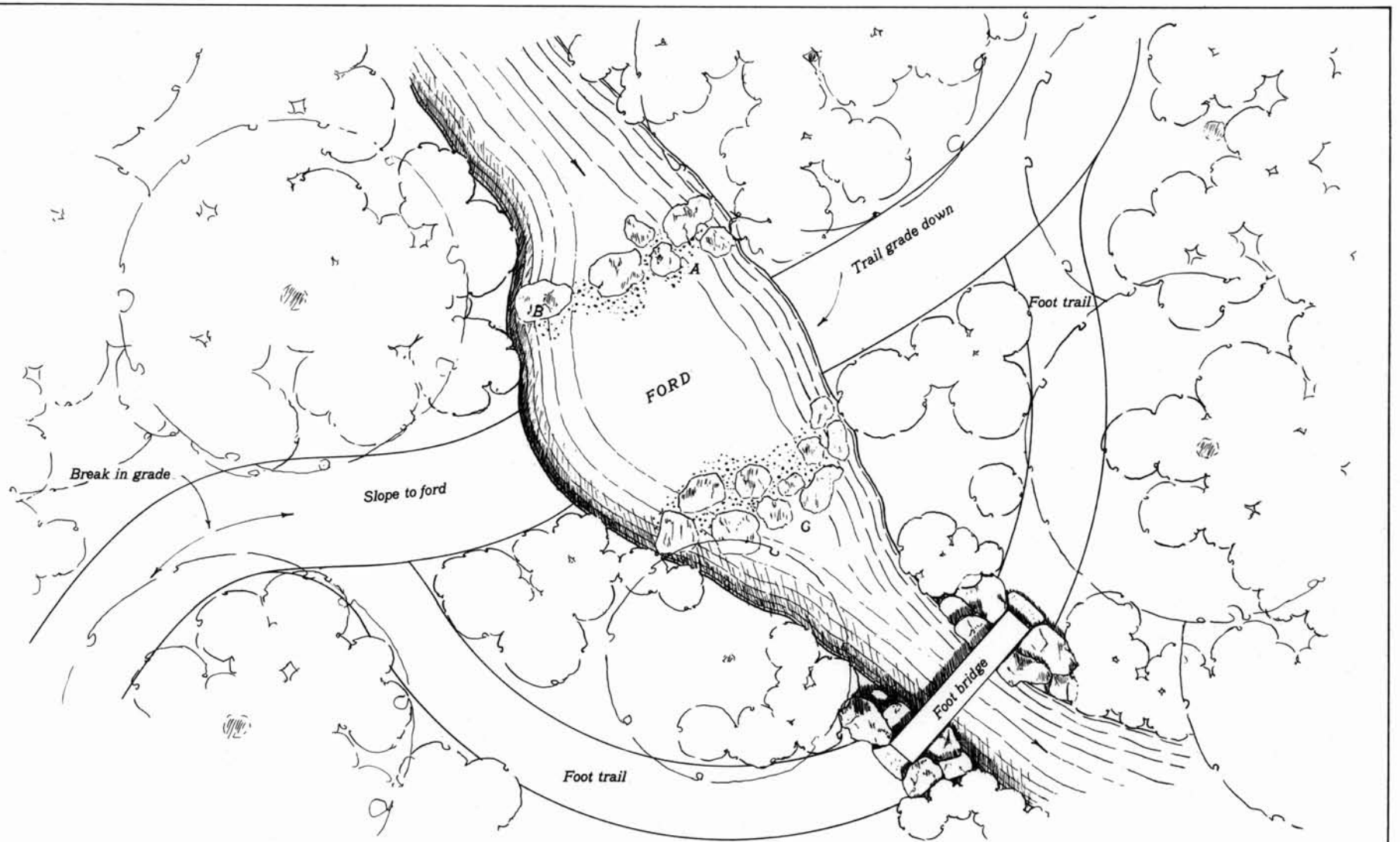
STREAM CROSSINGS FOR HORSE AND FOOT TRAILS SKETCH NO. 19
